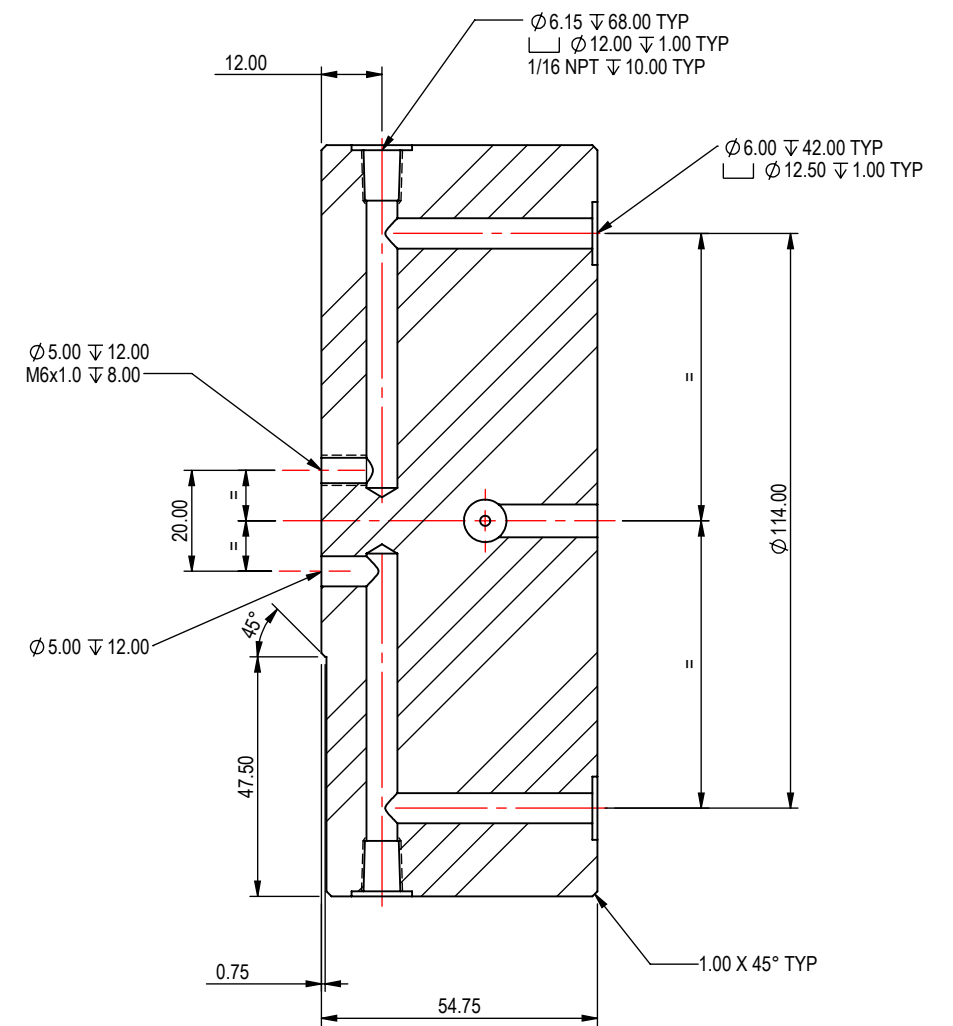
SECTION B-B
